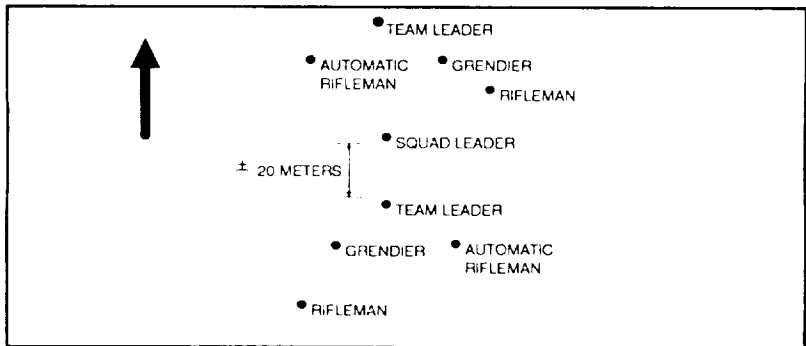
Figure 2-19. Squad traveling.
